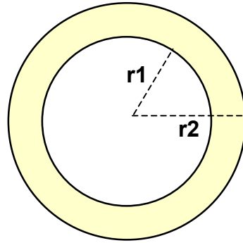
Circular Ring (Annulus)
