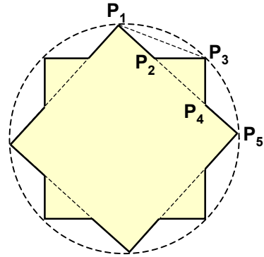
Star Polygon (n=8, k=2)
