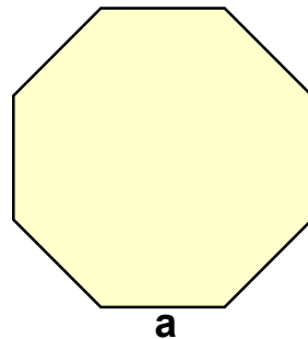
Regular Polygon (n=8)
