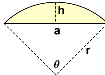
Segment of a Circle
